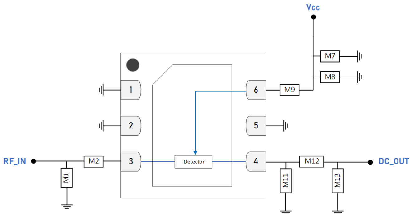
GRF1201 Standard Evaluation Board Schematic
