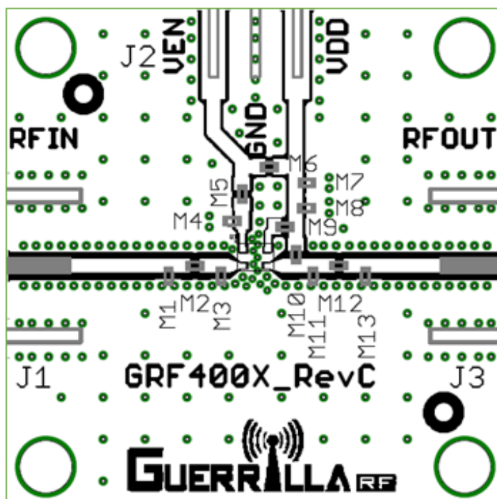
GRF1201 Evaluation Board Assembly Diagram
