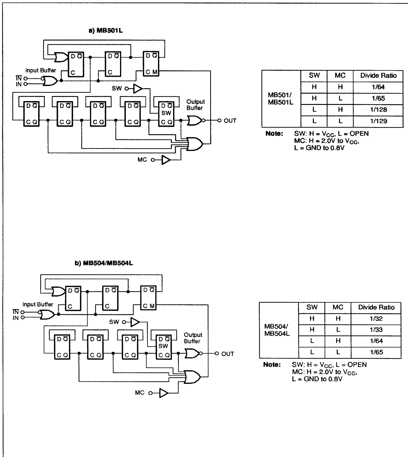
Figure 1. Block Diagrams
