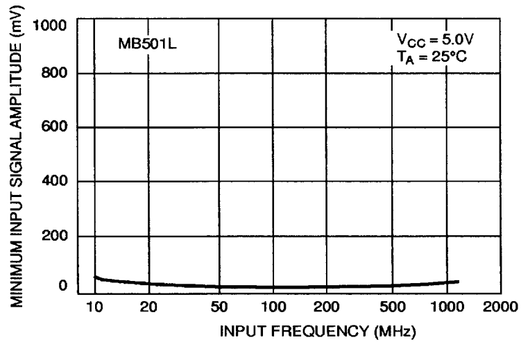
Figure 3. Input Signal Amplitude vs. Input Frequency
