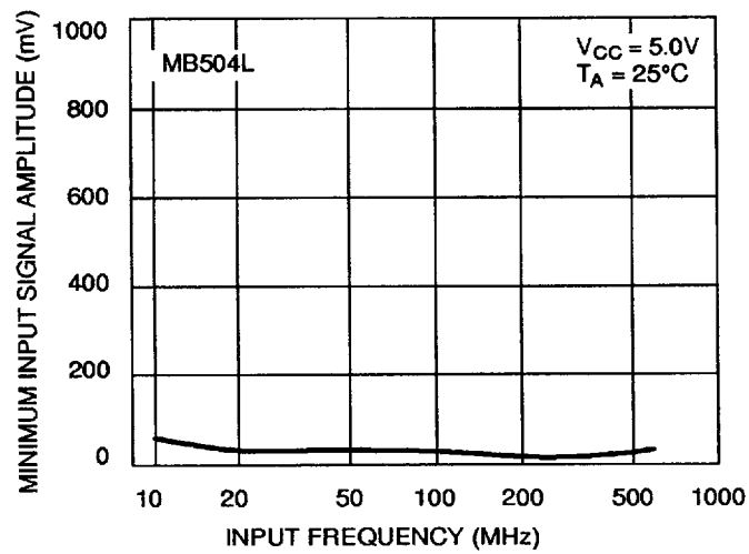
Figure 5. Input Signal Amplitude vs. Input Frequency
