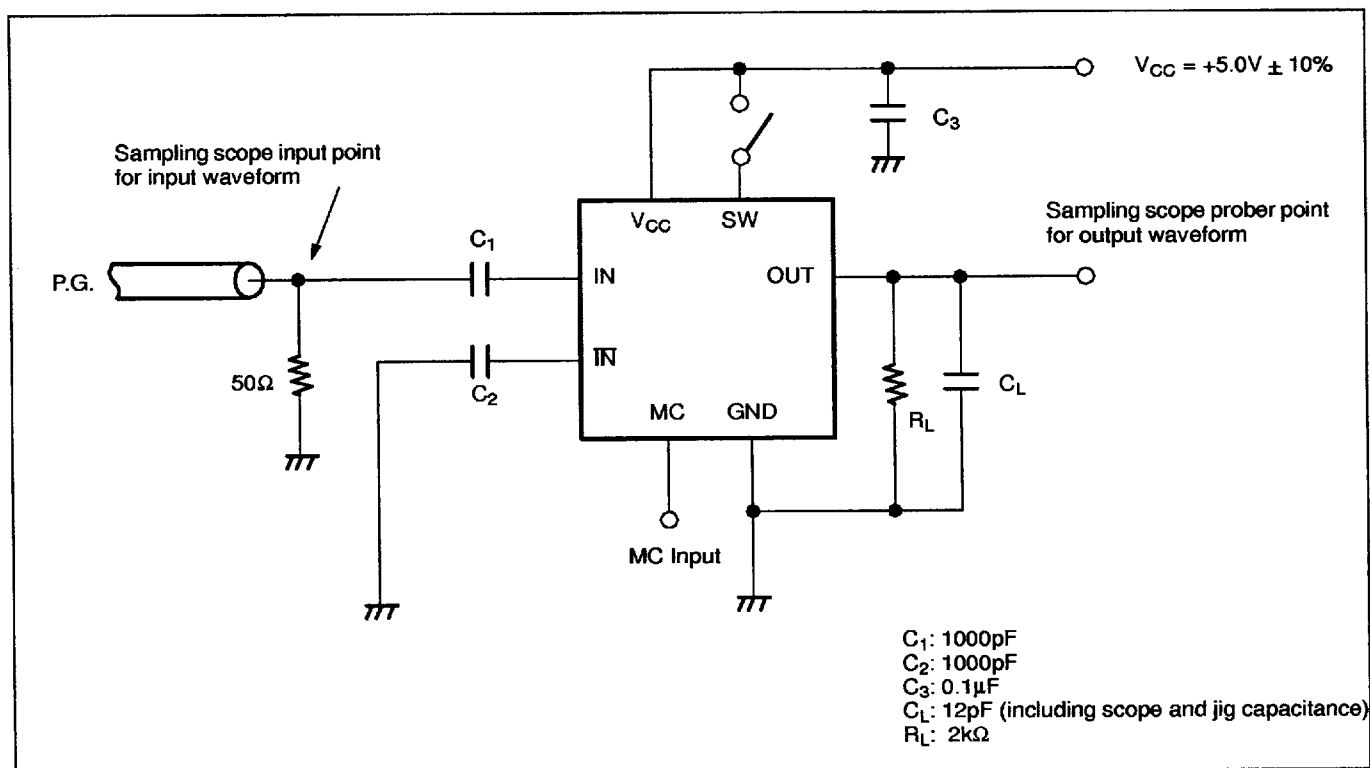
Figure 2. Test Circuit
