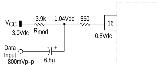
Figure 29. Analog AM Transmitter
