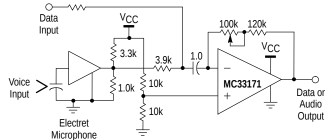
Figure 17. Microphone Amplifier
