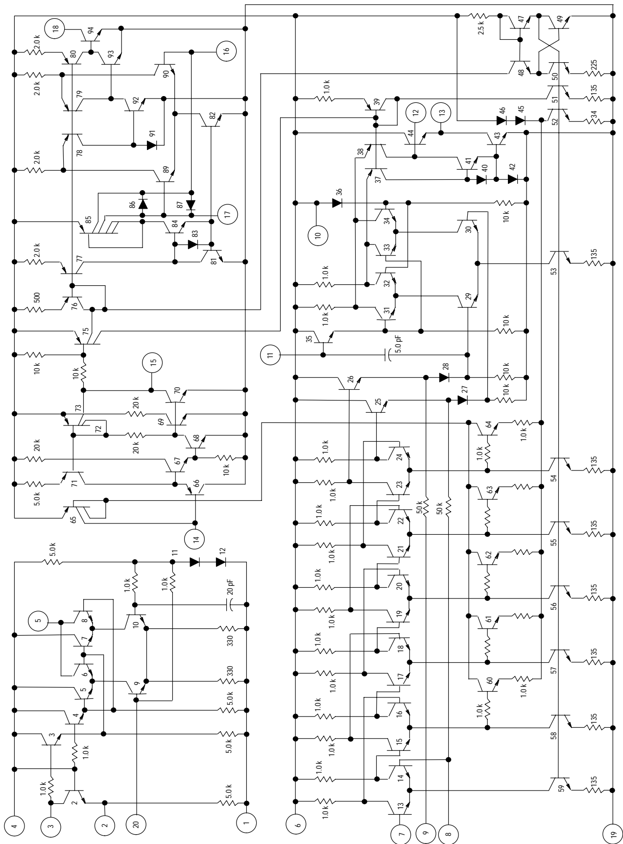
Figure 7. Internal Schematic
