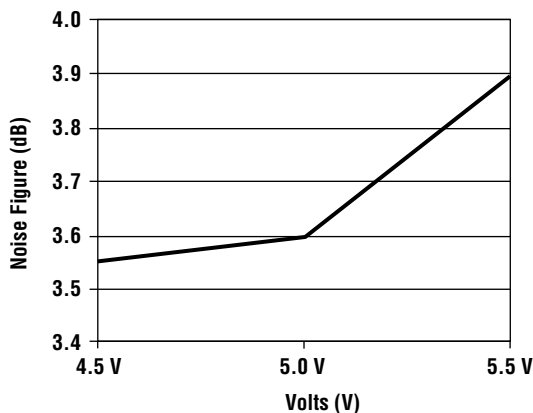
Rx Noise Figure vs. V_{DD}
