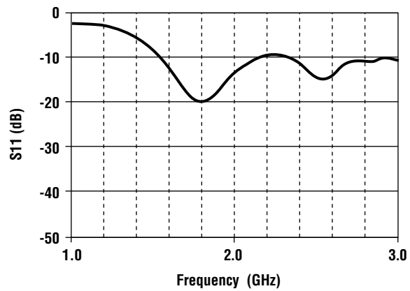
|S11| vs. Frequency
