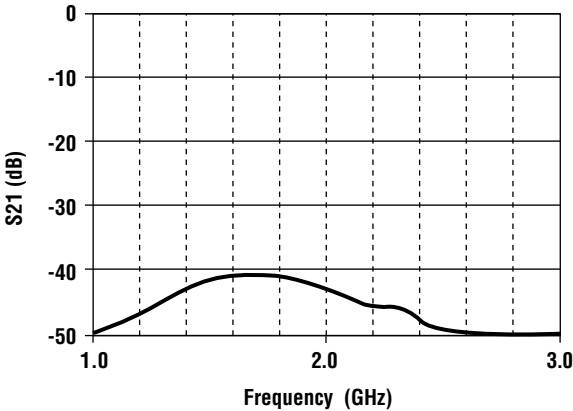
|S21| vs. Frequency
