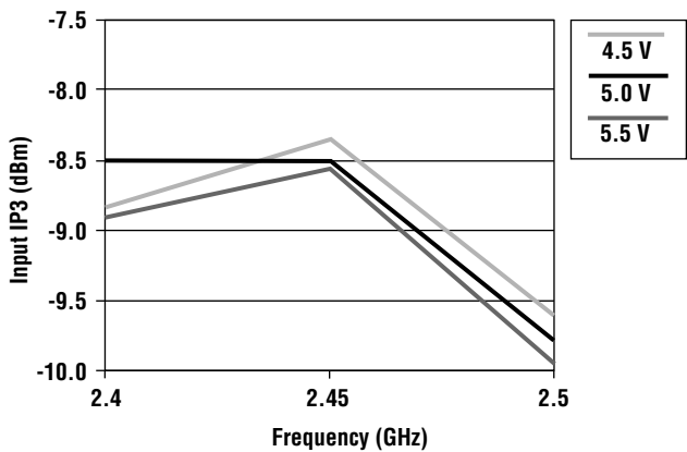
Rx Input IP3 vs. Frequency vs. V_{DD}
