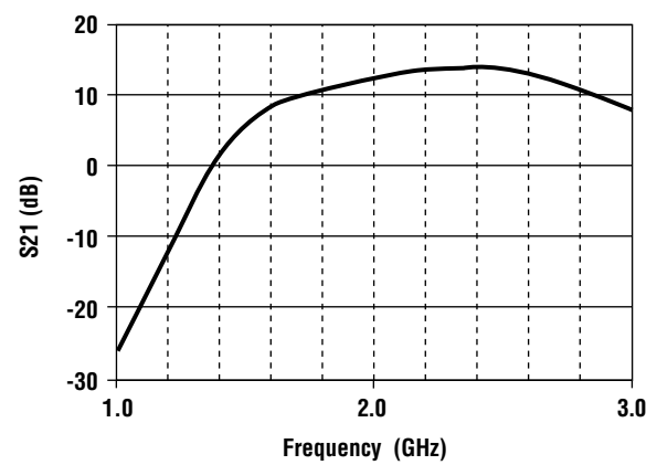
|S21| vs. Frequency
