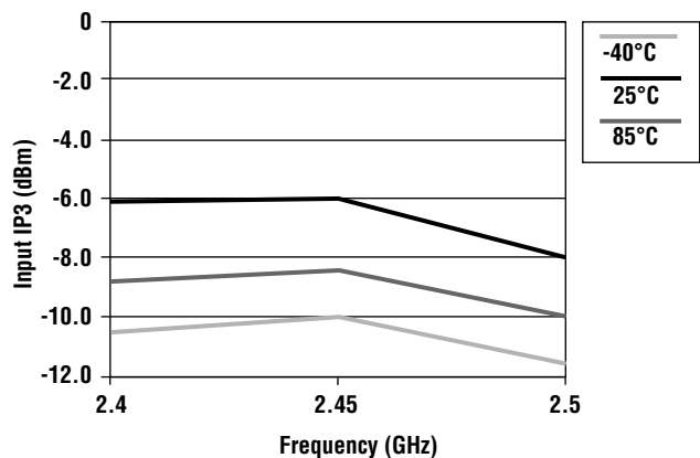
Rx Input IP3 vs. Frequency vs. Temp.
