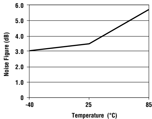
Rx Noise Figure vs. Temperature
