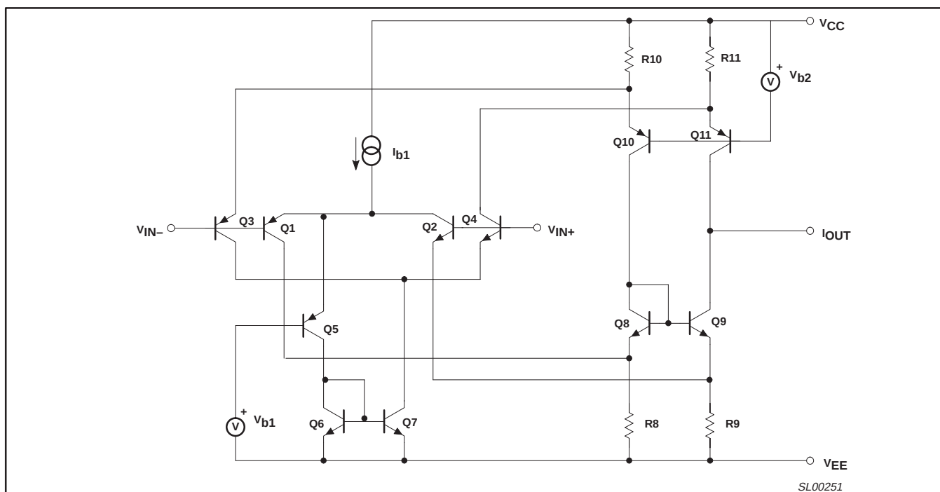
Figure 2. Input Stage
