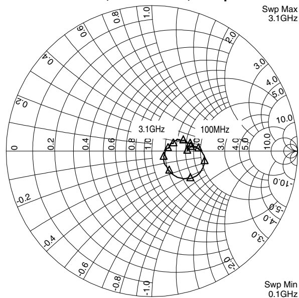
RF2323 S22, Vcc = 2.7 V, Temp = 25°C
