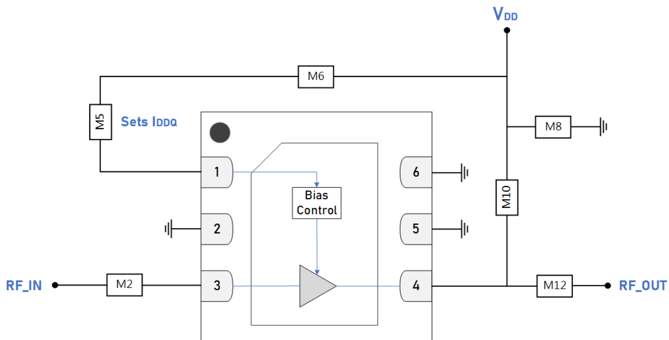
GRF2012W Standard Evaluation Board Schematic
