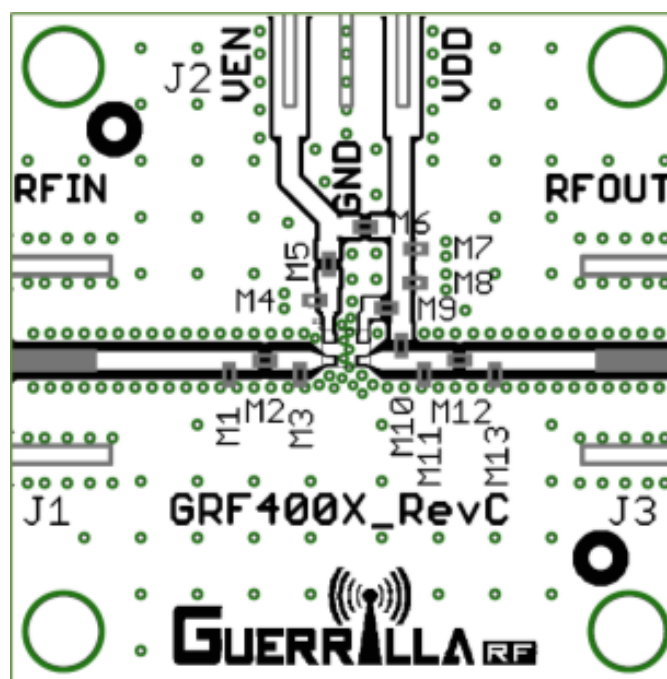
GRF2012W Evaluation Board Assembly Diagram
