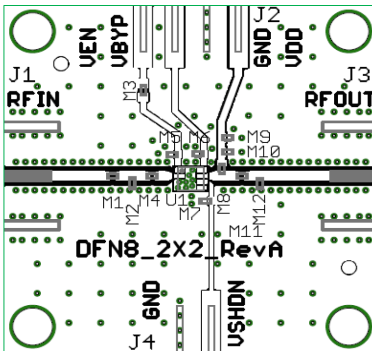
GRF2070 Evaluation Board Assembly Diagram
