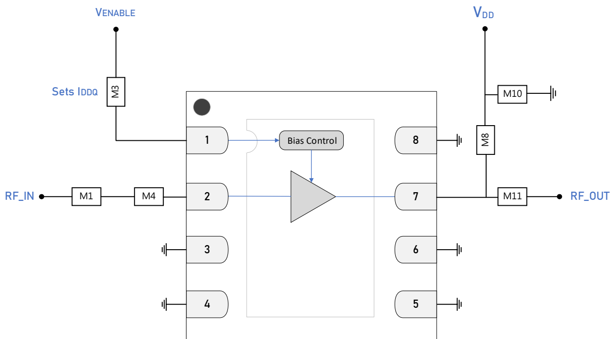
GRF2070 Standard Evaluation Board Schematic
