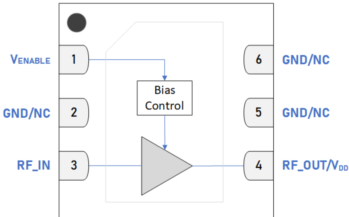
Pin Out (Top View)
