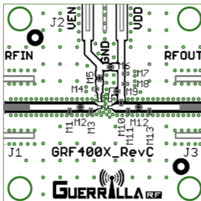
GRF2105W Evaluation Board Assembly Diagram
