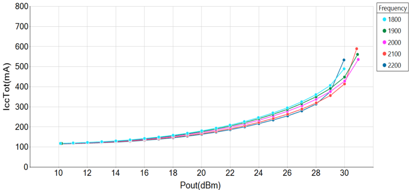
GRF5219 IccTot vs Pout at Temp = 25 degC and Vcc3(V) = 5 V
