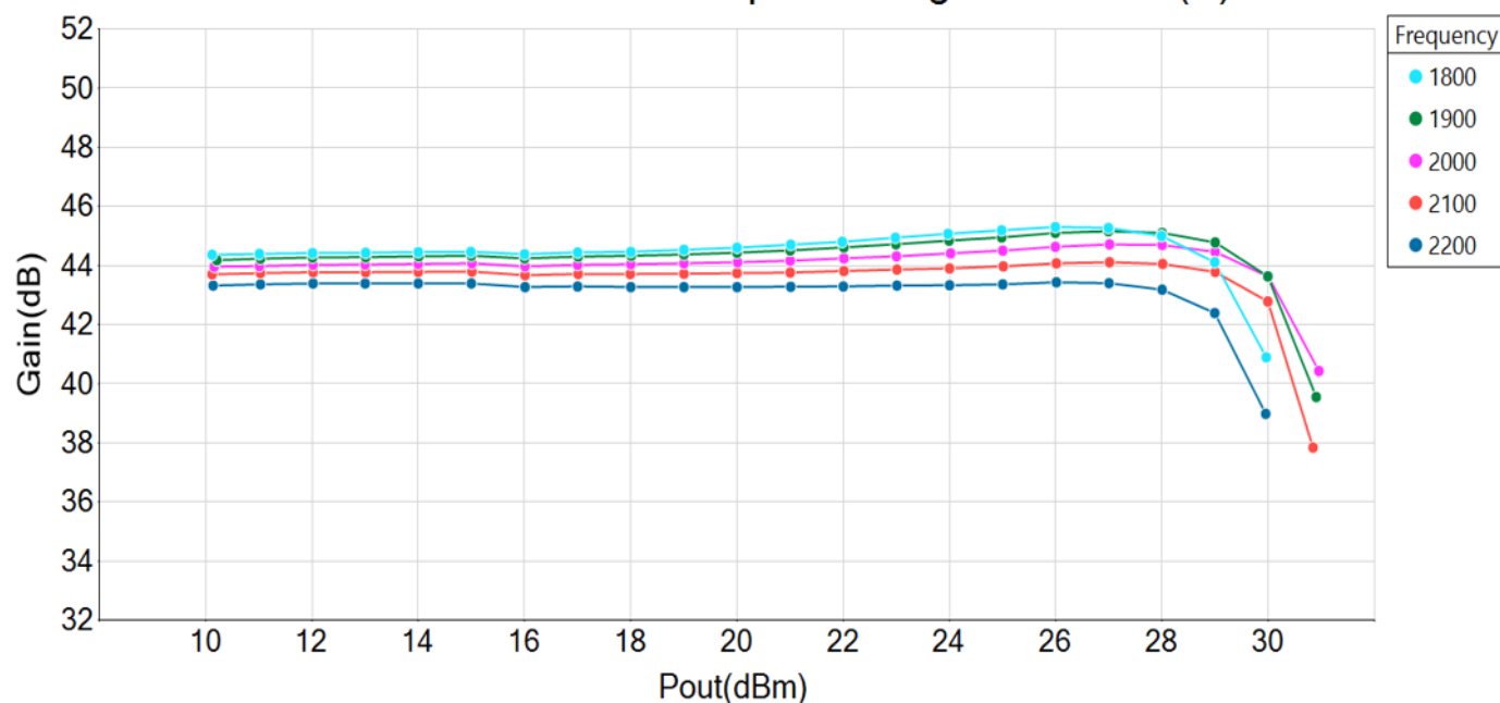
GRF5219 Gain vs Pout at Temp = 25 degC and V_{cc3}(V) = 5\text{ V}
