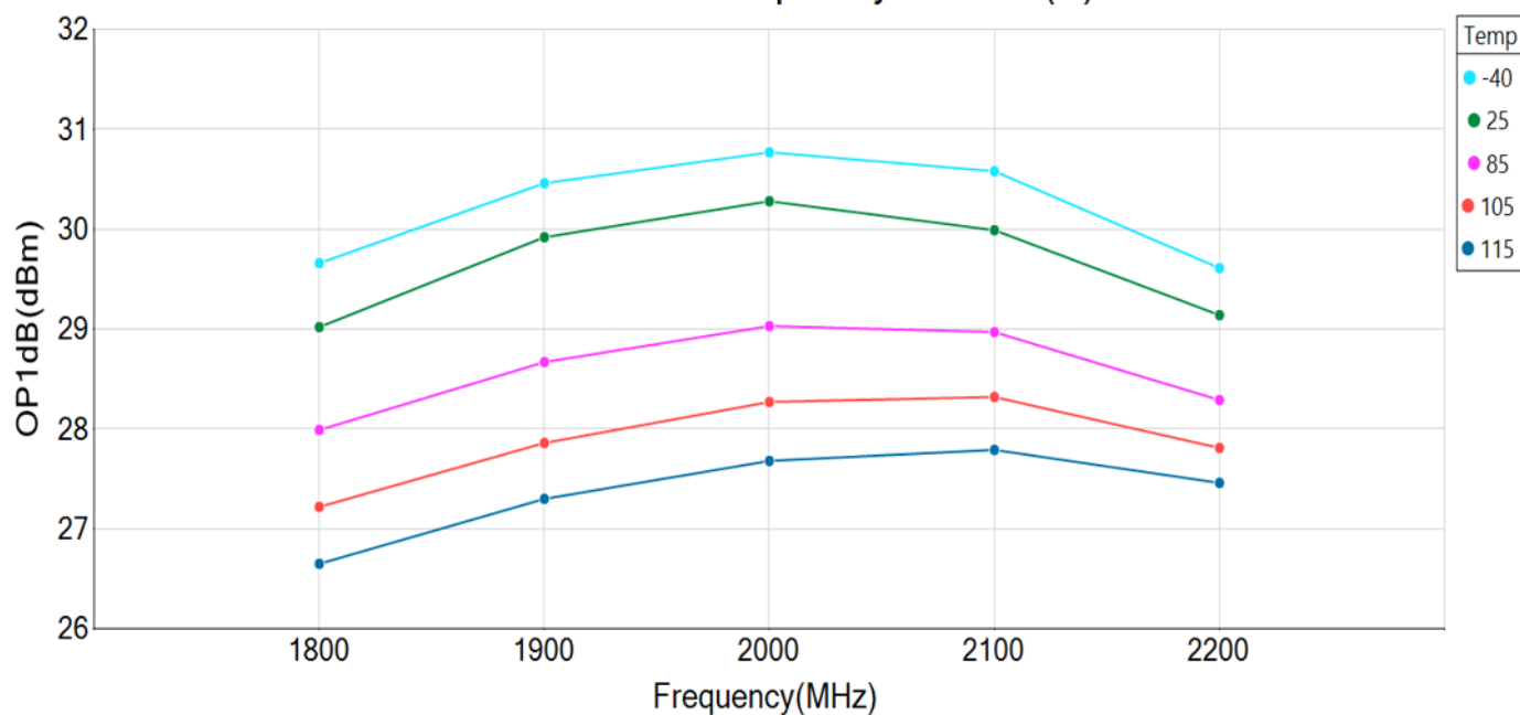
GRF5219 OP1dB vs Frequency at Vcc3(V) = 5 V
