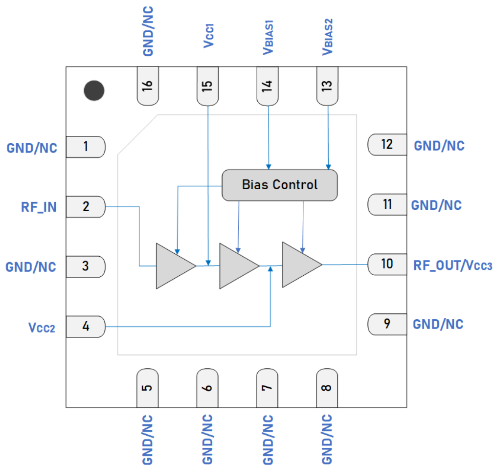
Pin Out (Top View)
