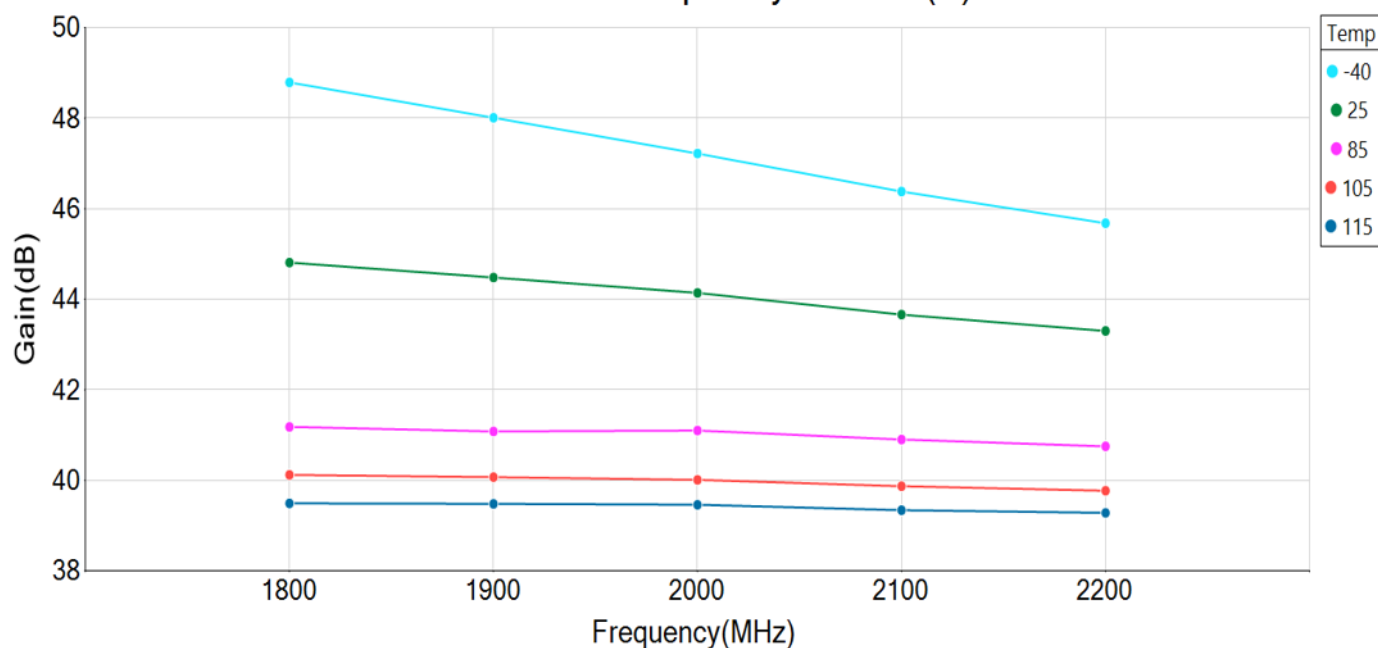
GRF5219 Gain vs Frequency at V_{cc3}(V) = 5\text{ V}
