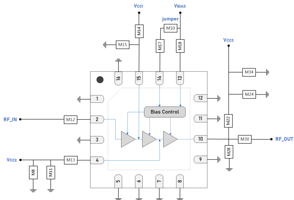
GRF5219 Standard Evaluation Board Schematic
