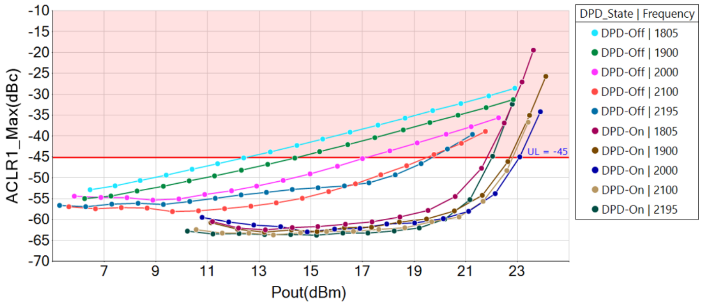
GRF5219 ACLR1 vs Pout at Vcc2 = 5 V and ModulationType = 5G_1x10MHz
