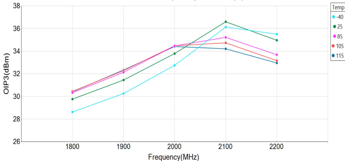
GRF5219 OIP3 vs Frequency at Vcc3(V) = 5 V
