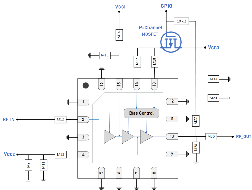
GRF5219 Recommended schematic for applications using low current GPIO to toggle V_{BIAS1} and V_{BIAS2}
