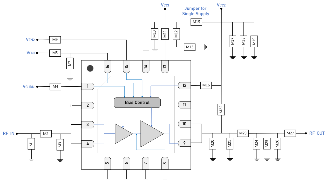
GRF5507 Standard Evaluation Board Schematic
