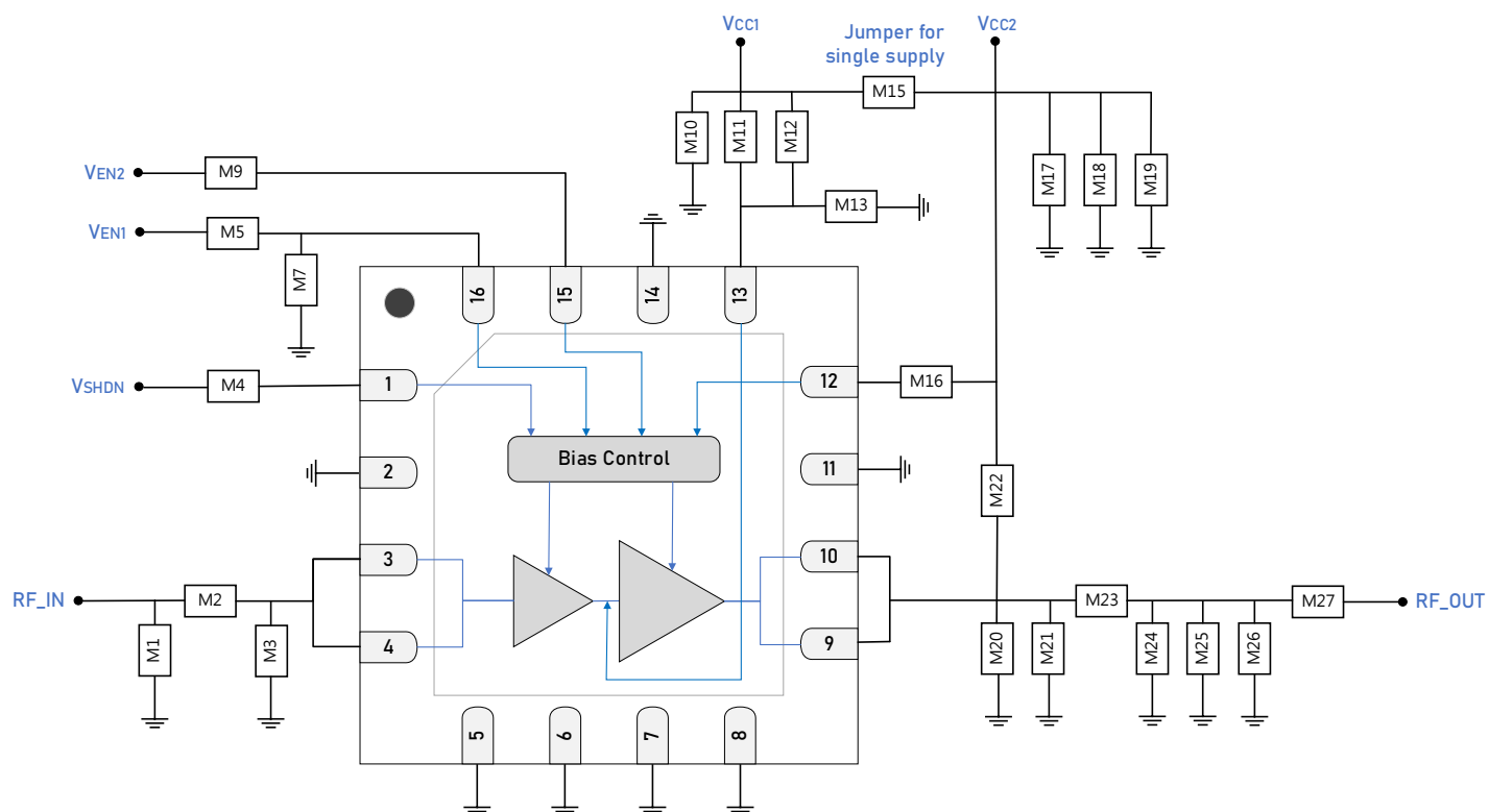
GRF5510 Standard Evaluation Board Schematic
