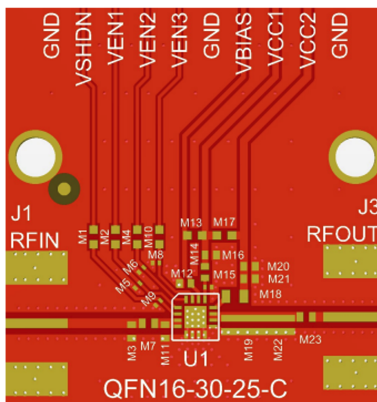
GRF5536W Evaluation Board Assembly Diagram
