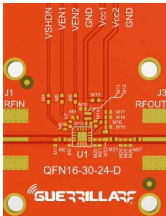
GRF5605 Evaluation Board Assembly Diagram
