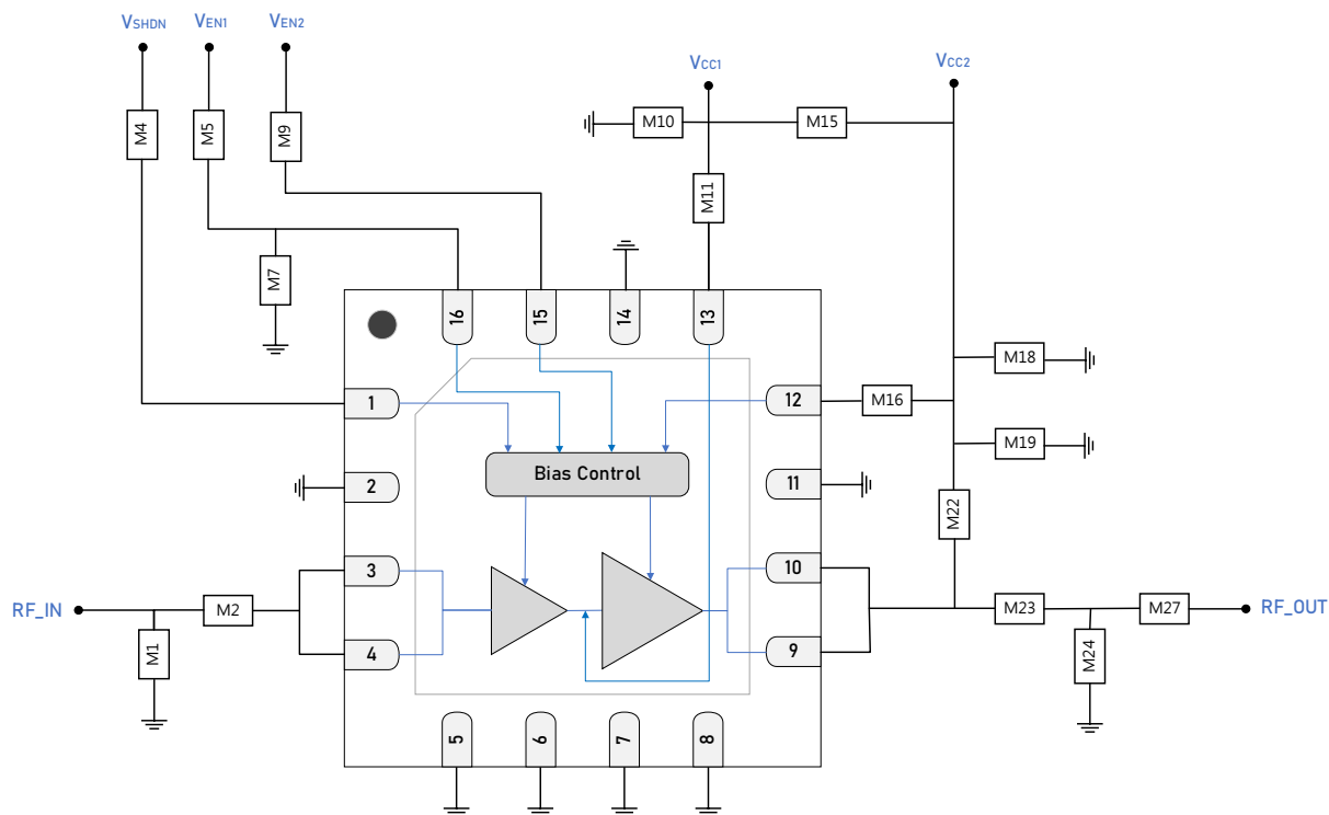
GRF5605 Standard Evaluation Board Schematic
