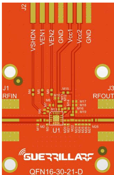
GRF5617 Evaluation Board Assembly Diagram
