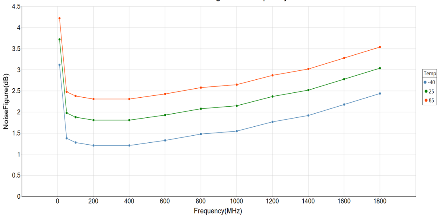
GRF7240 Noise Figure vs Frequency
