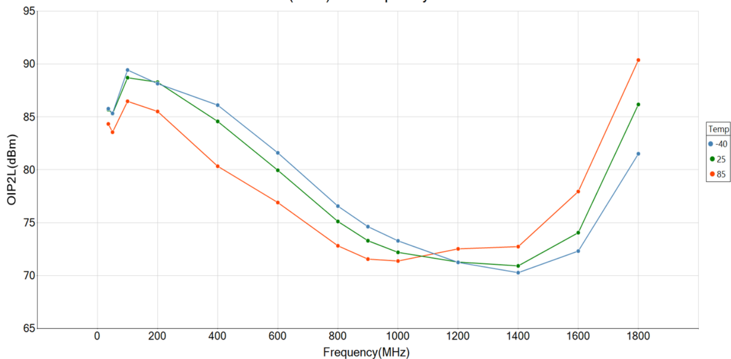
GRF7240 OIP2L(dBm) vs Frequency at Pout = 12 dBm
