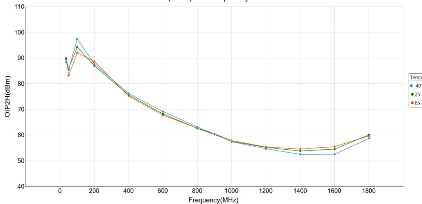
GRF7240 OIP2H(dBm) vs Frequency at Pout = 12 dBm
