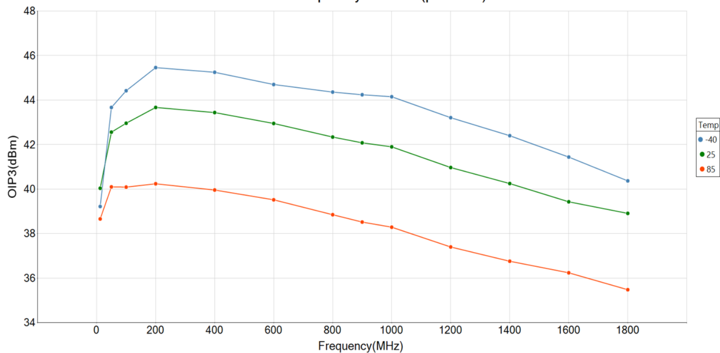
GRF7240 OIP3 vs Frequency at Pout (per tone) = 12 dBm
