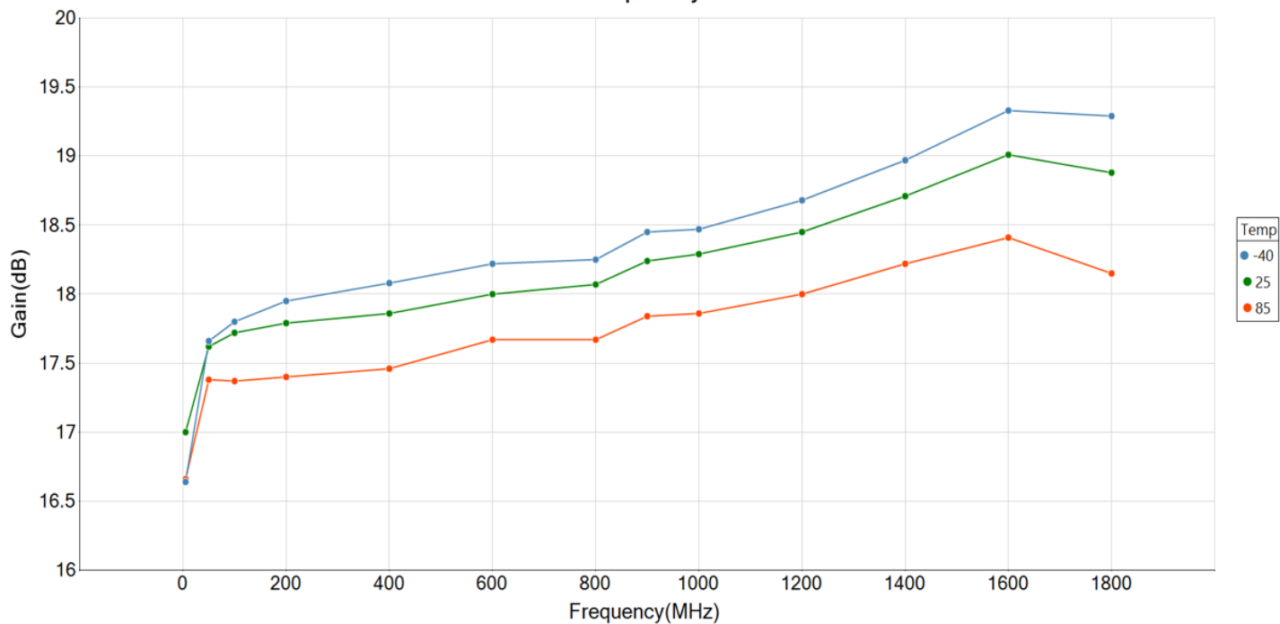
GRF7240 Gain vs Frequency at Pin = -25 dBm
