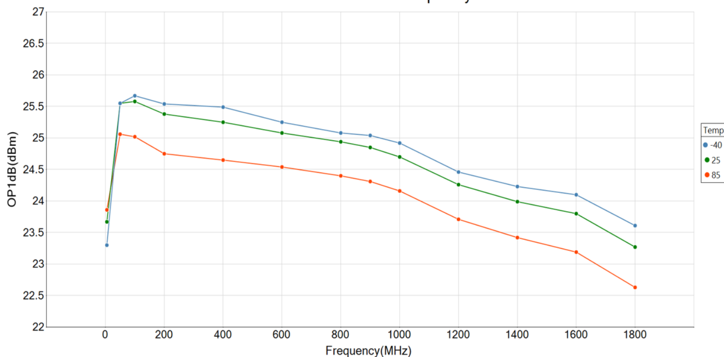
GRF7240 OP1dB vs Frequency
