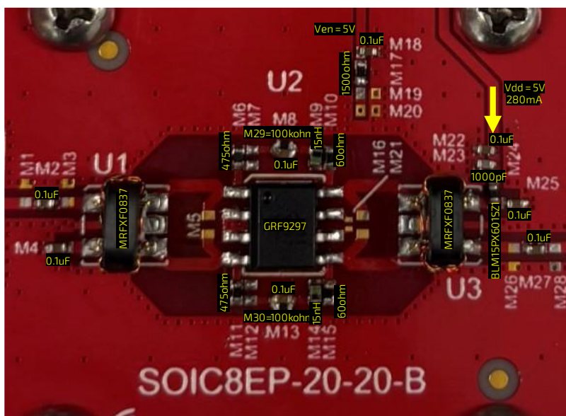
GRF9297 Evaluation Board Assembly Diagram
