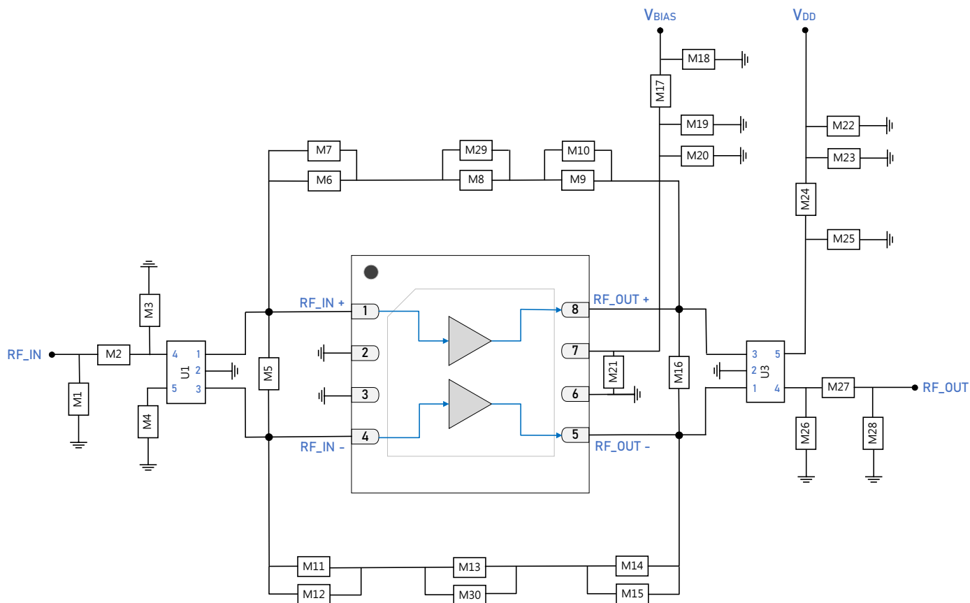
GRF9297 Standard Evaluation Board Schematic
