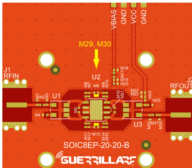
GRF9811 Evaluation Board Assembly Diagram
