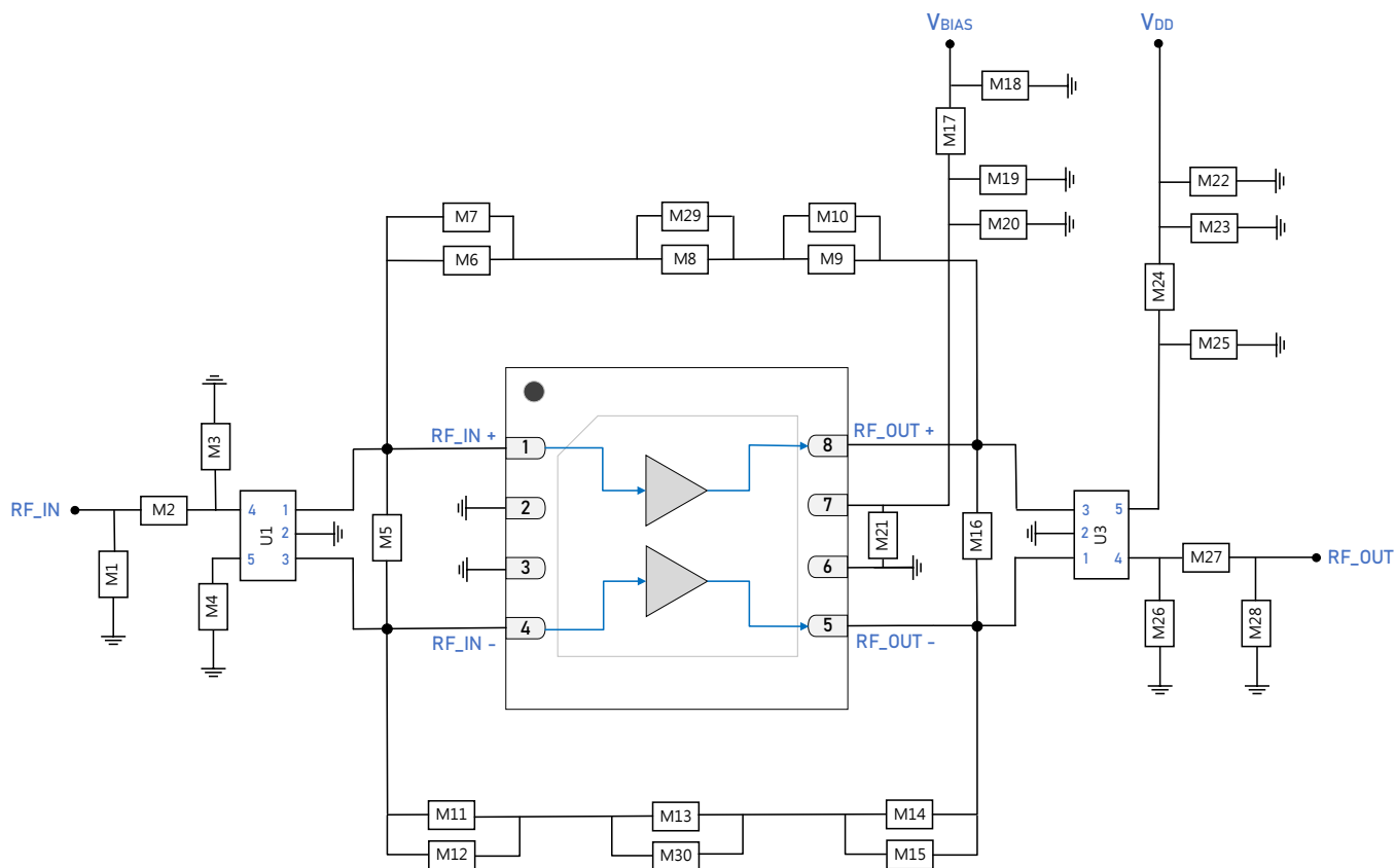
GRF9811 Standard Evaluation Board Schematic
