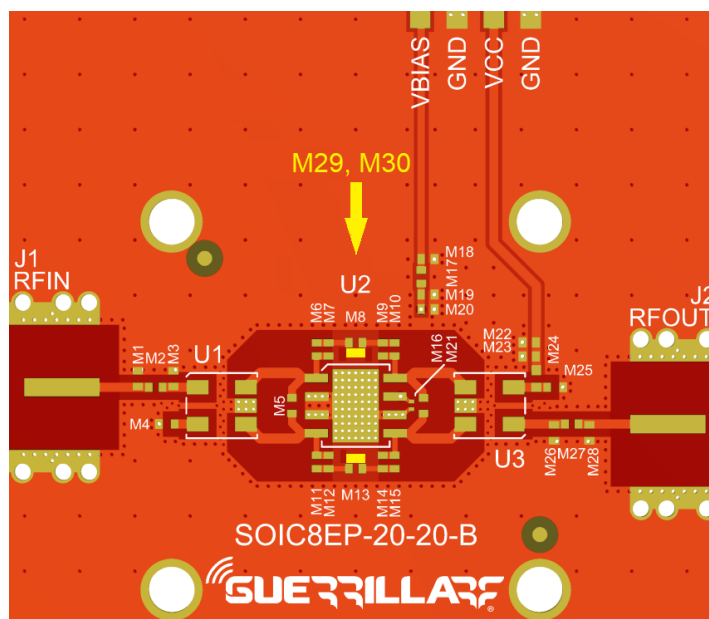
GRF9834 Evaluation Board Assembly Diagram
