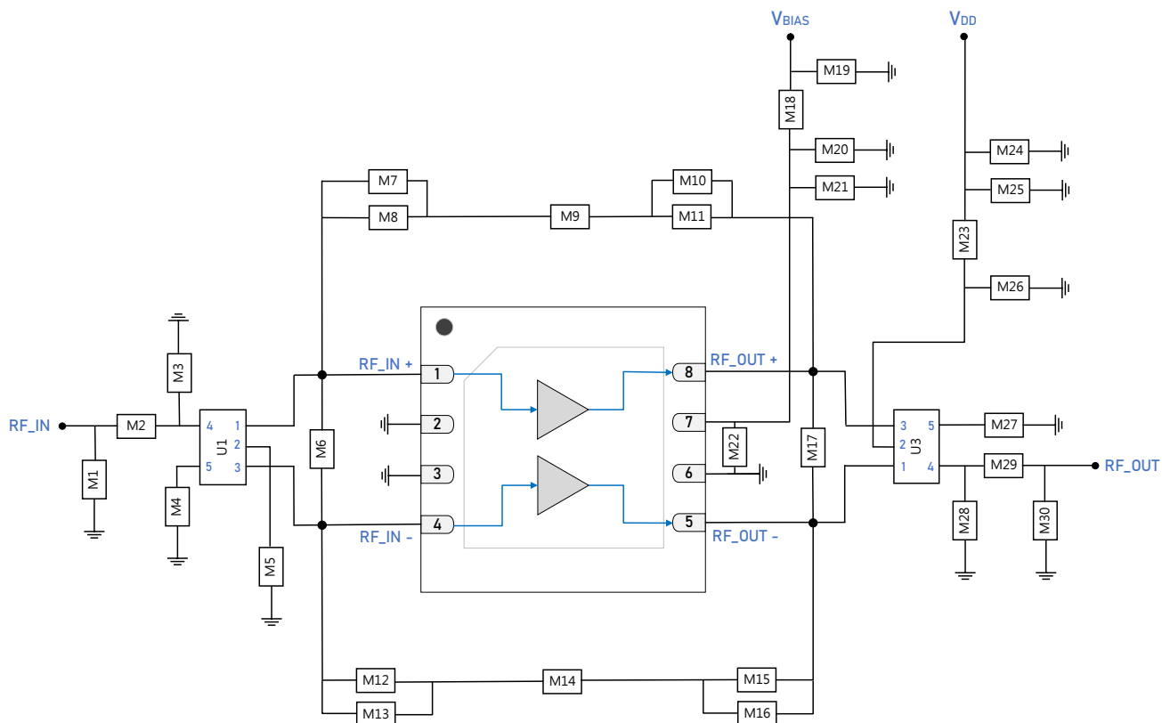
GRF9897 Standard Evaluation Board Schematic
