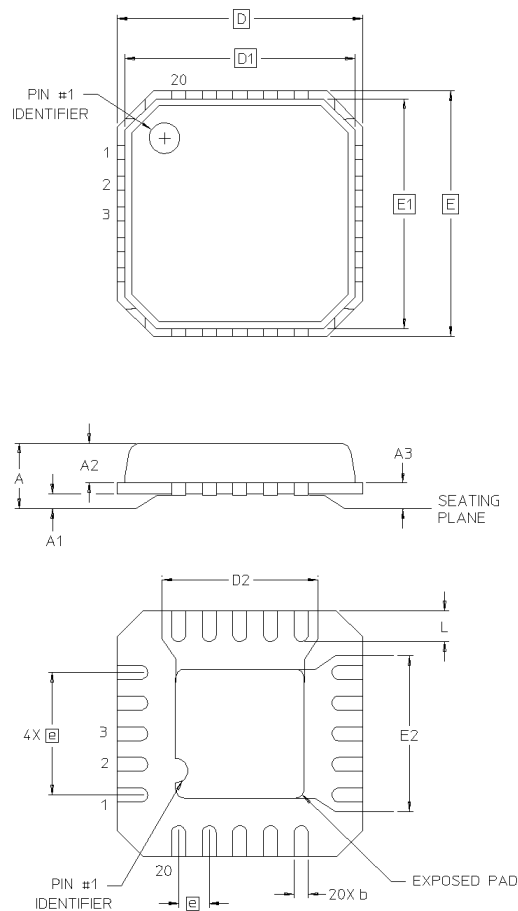
5 mm FQFP-N 20 Lead Anvil Singulated
