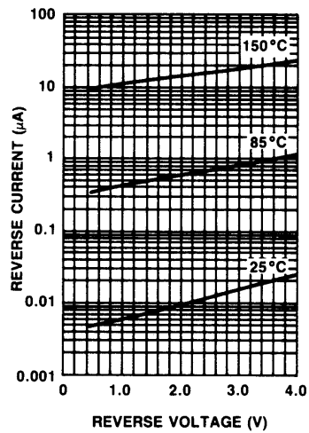
REVERSE CURRENT vs REVERSE VOLTAGE (MA4CS102)
