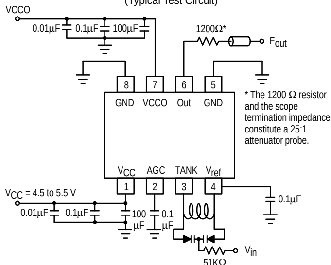
BLOCK DIAGRAM (Typical Test Circuit)
