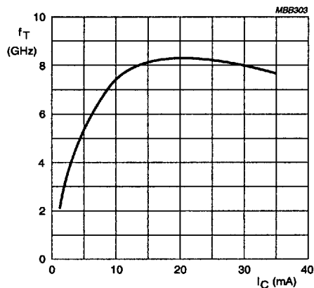
Fig.5 Transition frequency as a function of collector current.
