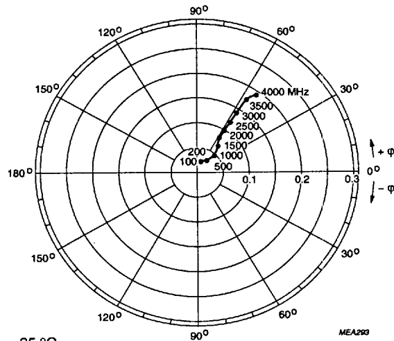
Fig.11 Common emitter reverse transmission coefficient ( S_{12} ).
