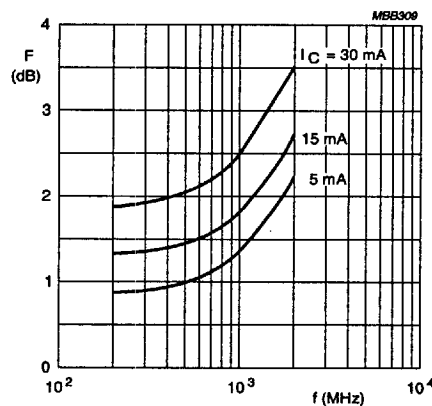
Fig.8 Minimum noise figure as a function of frequency.
