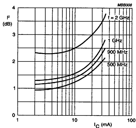
Fig.7 Minimum noise figure as a function of collector current.
