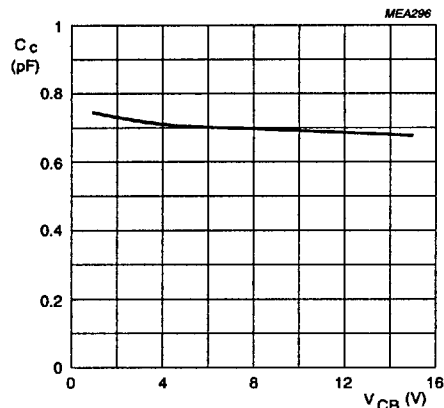
Fig.4 Collector capacitance as a function of collector-base voltage.
