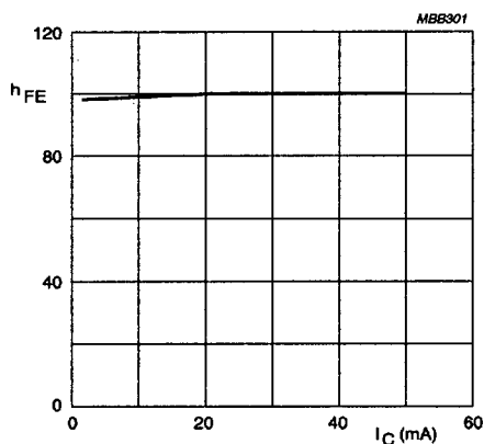
Fig.3 DC current gain as a function of collector current.
